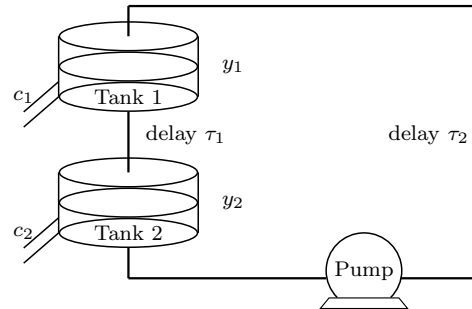
Fig. 1. A water flow system
